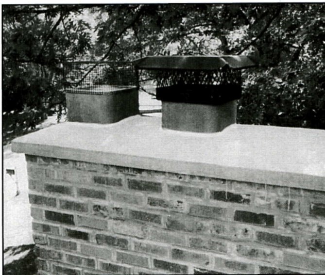
A freshly poured concrete crown is set to protect this masonry chimney for years to come.
